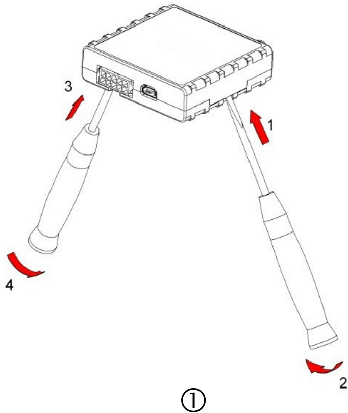
① Gently open GE-AM ECO case using screwdrivers
